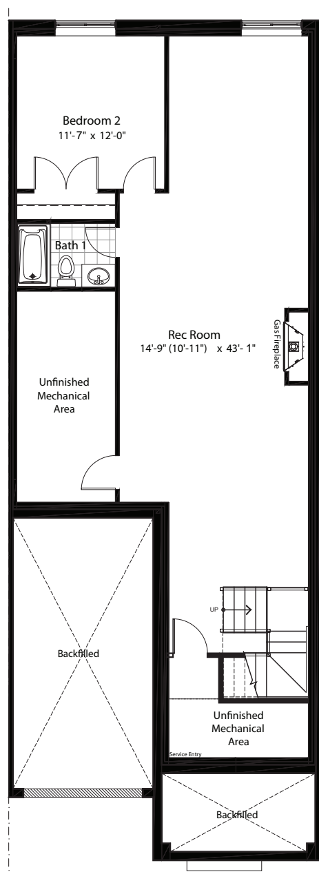
basement
