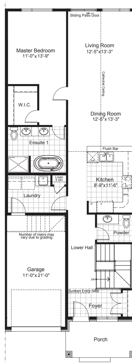
ground
